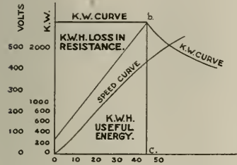
FIG. 4—ENERGY LOSS SERIES RESISTANCE
